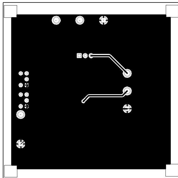
Figure 7. Bottom Copper Layer (Bottom View)
