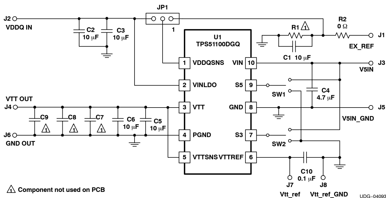
Figure 1. TPS51100EVM Schematic
