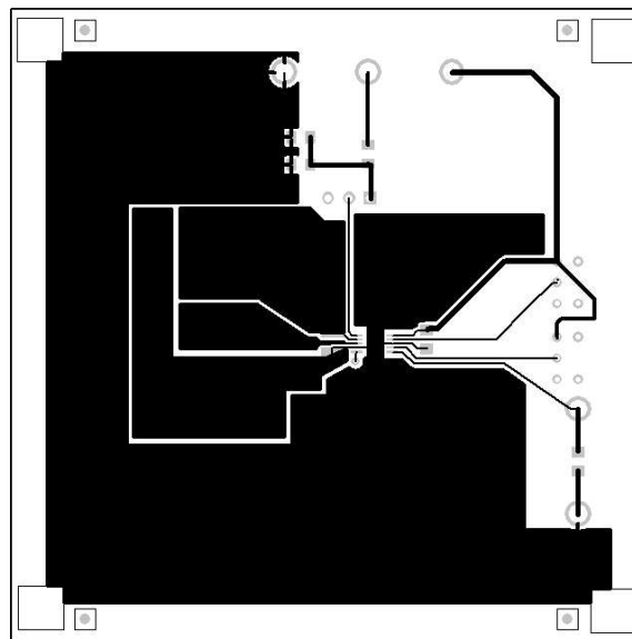
Figure 6. Top Copper Layer (Top View)
